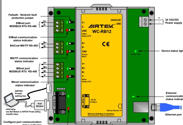
Figure 3. WC-RB12 wiring
