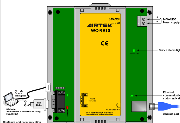
Figure 1. WC-RB10 wiring
