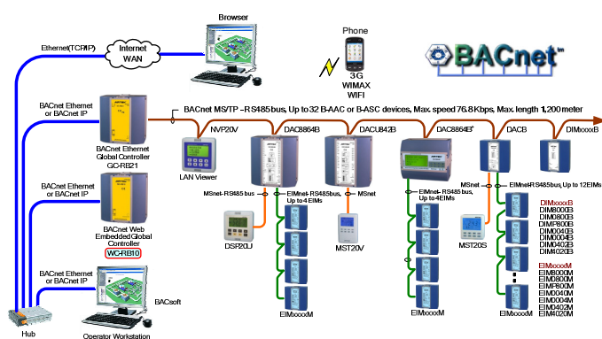
Figure 4. WC-RB10 network architecture
