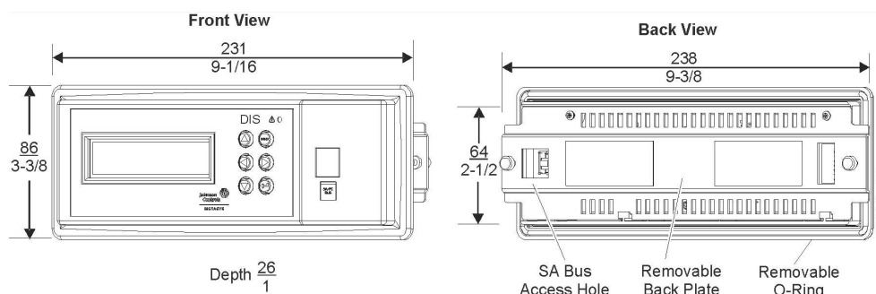
Figure 1. DIS1710 Mounting Dimensions, mm/in.
