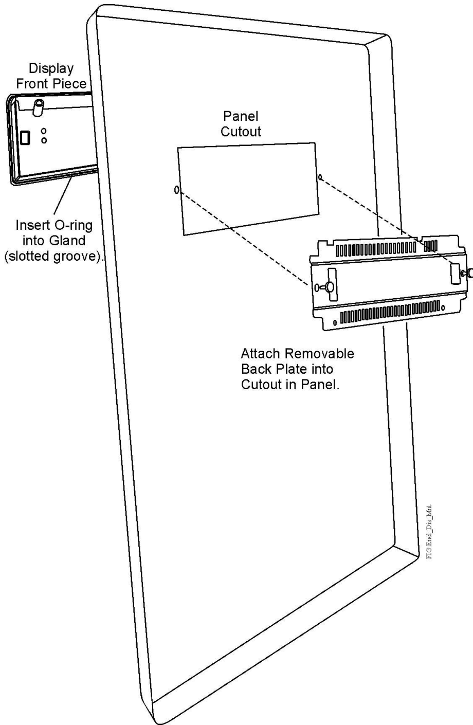
Figure 1. Attaching the display into panel cutout
